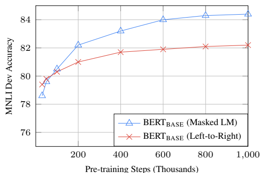
Figure 5: Ablation over number of training steps. This shows the MNL Dev accuracy after fine-tuning, starting from model parameters that have been pre-trained for k steps. The x-axis is the value of k .
